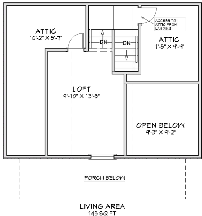
Upper Level
