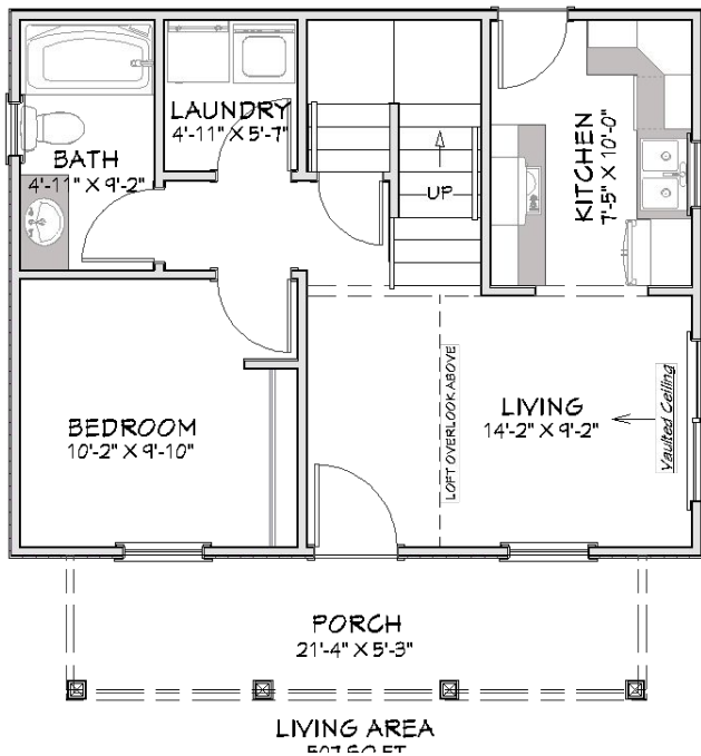
Main Level
